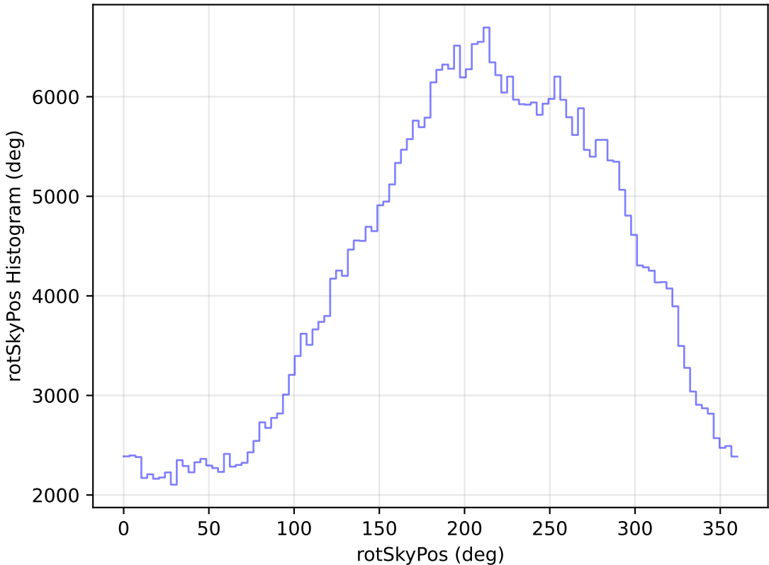
too_elab_r8_d2_griz_v3.4_10yrs WFD z band: rotSkyPos Histogram
