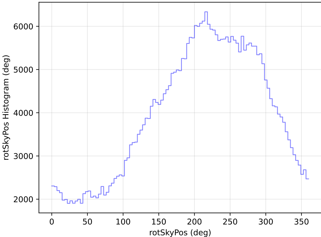
too_elab_r8_d2_griz_v3.4_10yrs WFD y band: rotSkyPos Histogram
