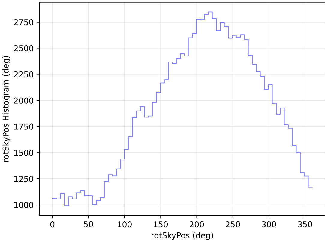
too_elab_r8_d2_griz_v3.4_10yrs WFD u band: rotSkyPos Histogram
