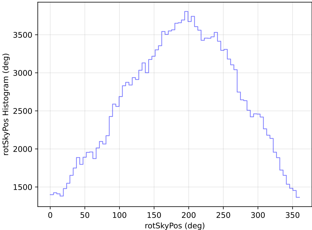
too_elab_r8_d2_griz_v3.4_10yrs WFD g band: rotSkyPos Histogram
