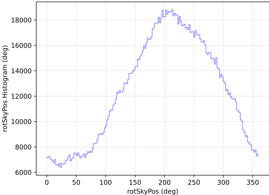
too_elab_r8_d2_griz_v3.4_10yrs WFD all bands: rotSkyPos Histogram
