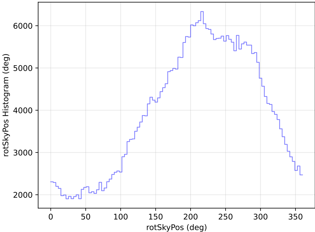
too_elab_r8_d2_griz_v3.4_10yrs All sky y band: rotSkyPos Histogram
