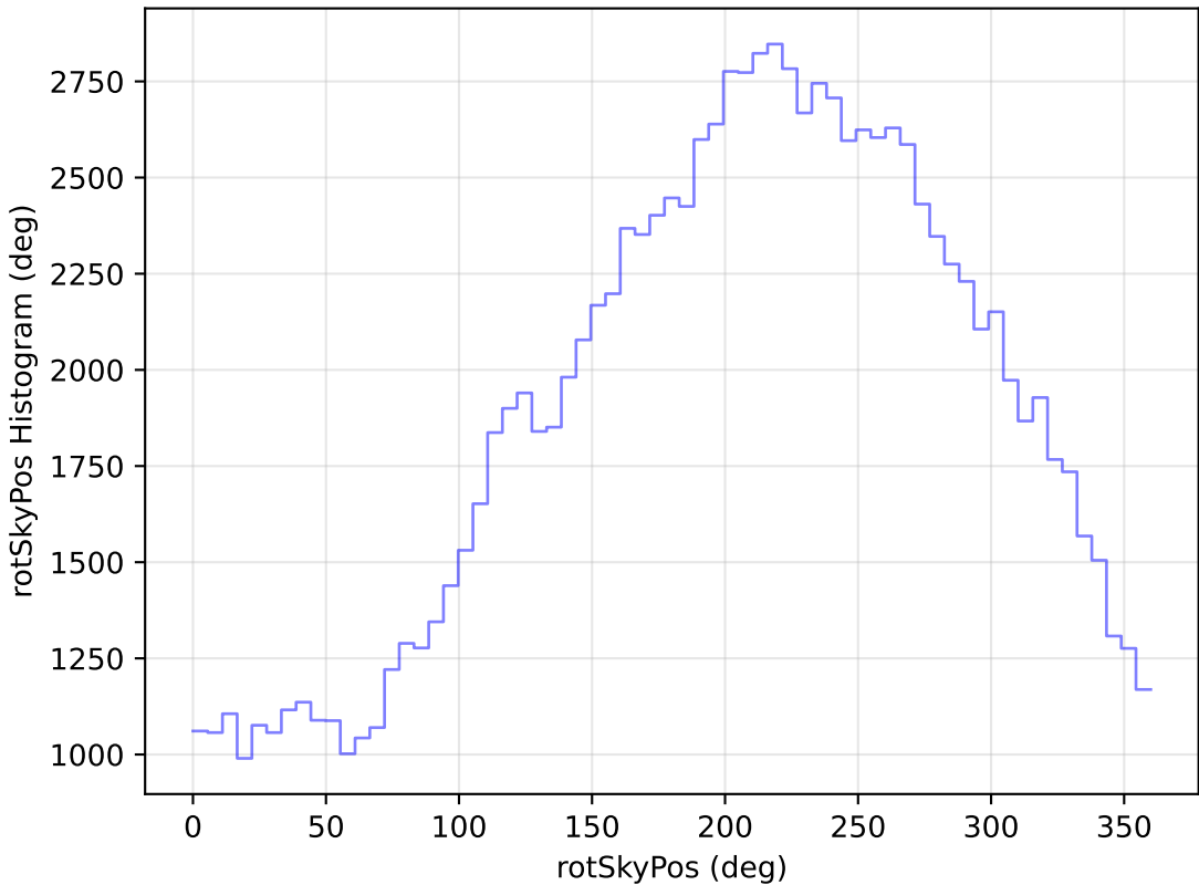
too_elab_r8_d2_griz_v3.4_10yrs All sky u band: rotSkyPos Histogram
