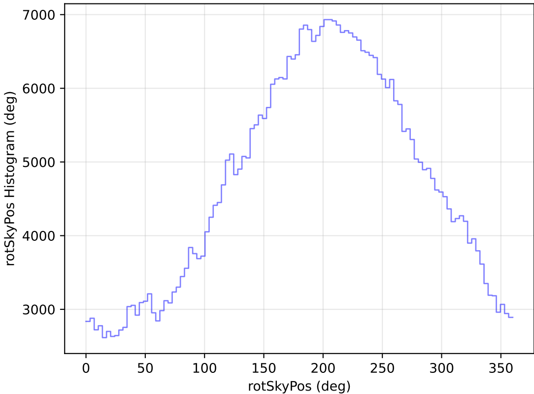
too_elab_r8_d2_griz_v3.4_10yrs All sky r band: rotSkyPos Histogram
