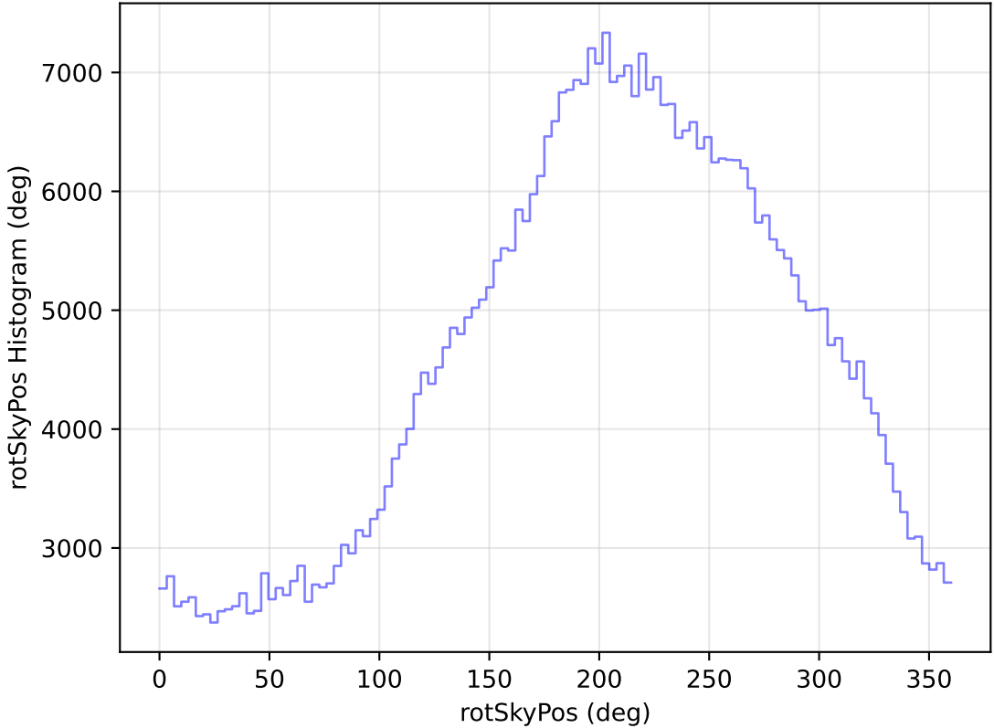
too_elab_r8_d2_griz_v3.4_10yrs All sky i band: rotSkyPos Histogram
