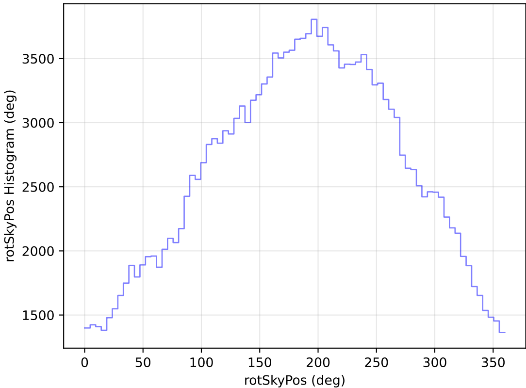
too_elab_r8_d2_griz_v3.4_10yrs All sky g band: rotSkyPos Histogram
