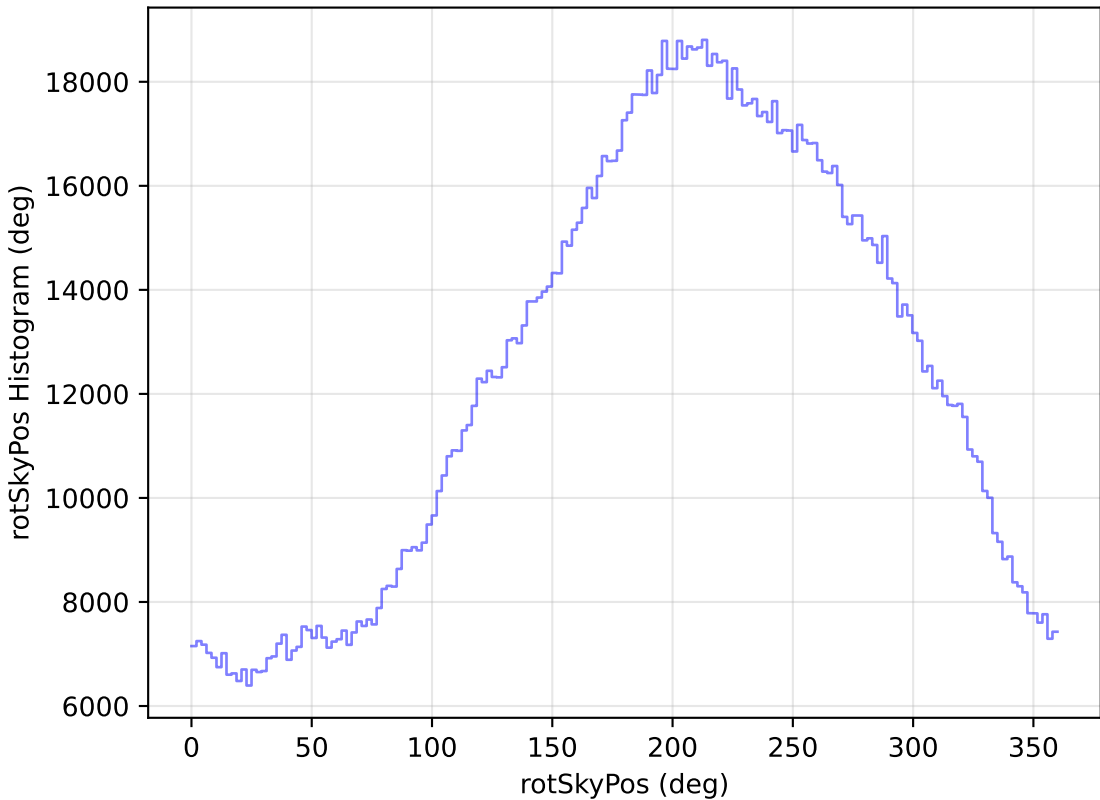
too_elab_r8_d2_griz_v3.4_10yrs All sky all bands: rotSkyPos Histogram
