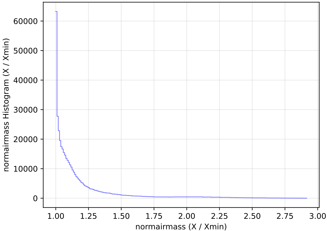
too_elab_r8_d2_griz_v3.4_10yrs WFD z band: normairmass Histogram
