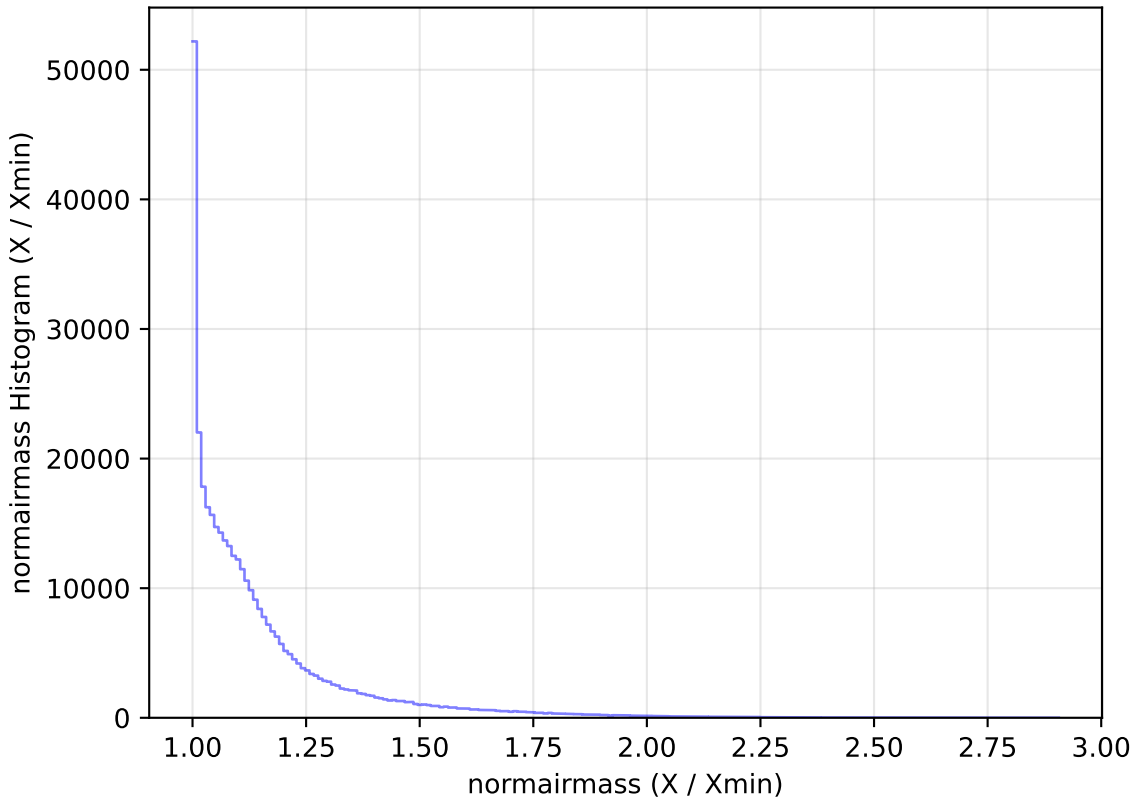
too_elab_r8_d2_griz_v3.4_10yrs WFD y band: normairmass Histogram
