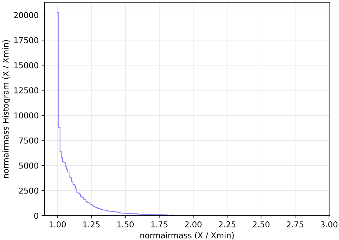
too_elab_r8_d2_griz_v3.4_10yrs WFD u band: normairmass Histogram
