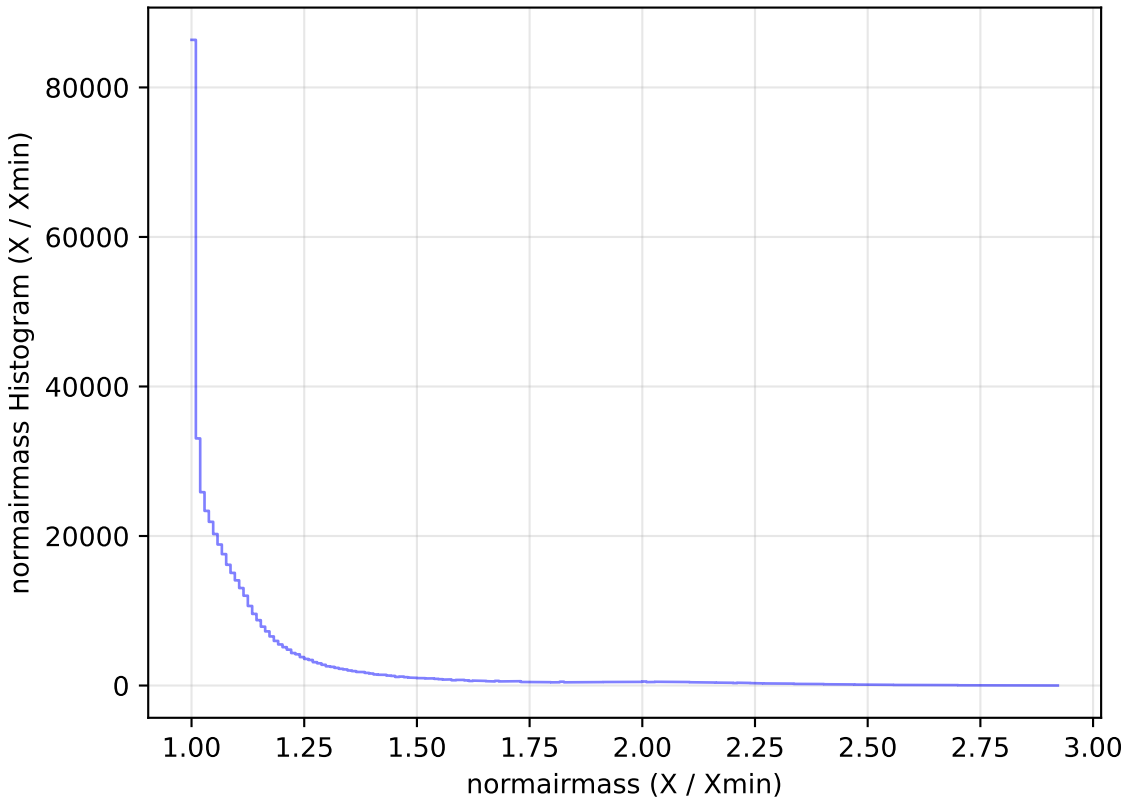
too_elab_r8_d2_griz_v3.4_10yrs WFD i band: normairmass Histogram
