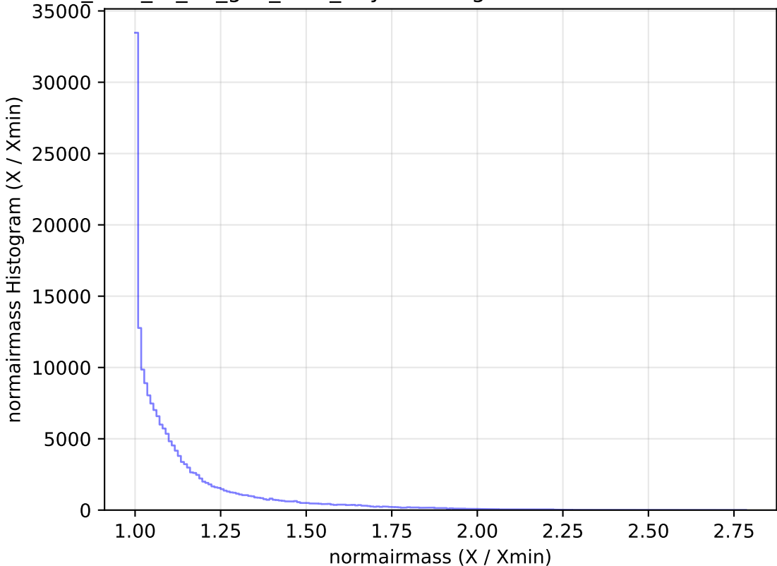
too_elab_r8_d2_griz_v3.4_10yrs WFD g band: normairmass Histogram
