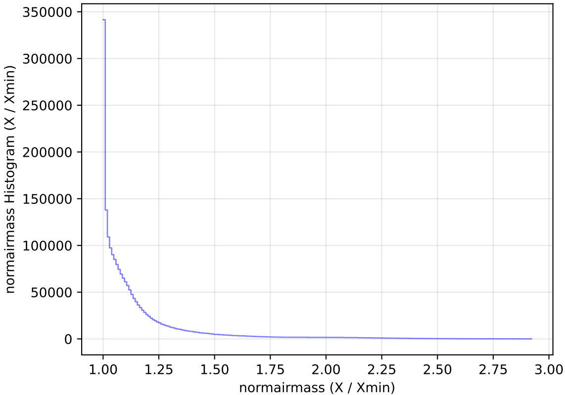
too_elab_r8_d2_griz_v3.4_10yrs WFD all bands: normairmass Histogram
