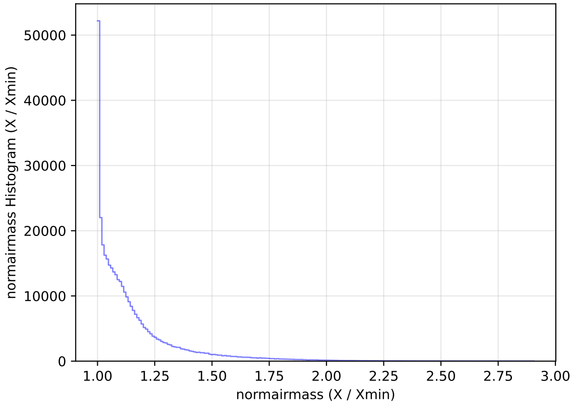
too_elab_r8_d2_griz_v3.4_10yrs All sky y band: normairmass Histogram
