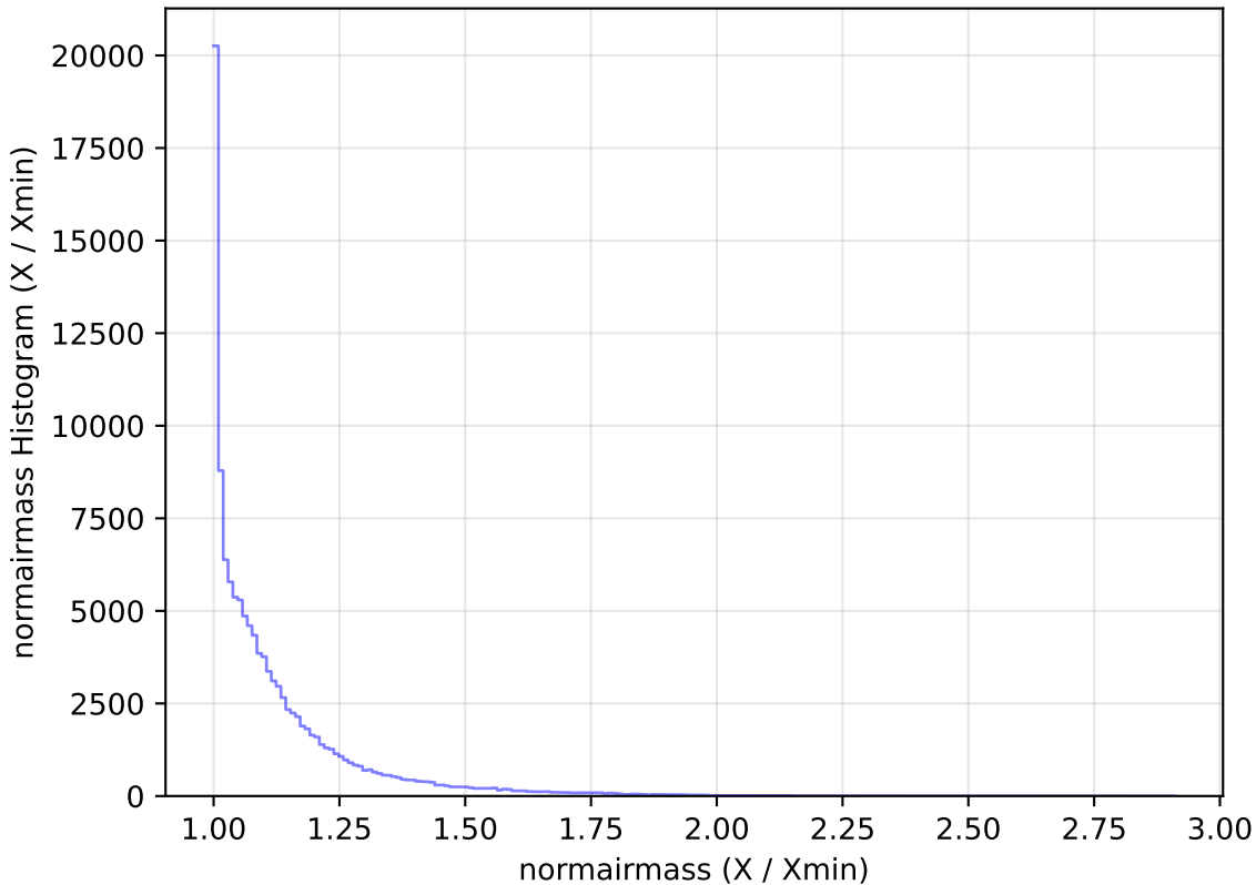
too_elab_r8_d2_griz_v3.4_10yrs All sky u band: normairmass Histogram
