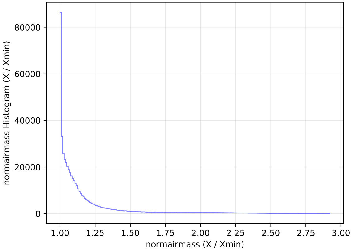
too_elab_r8_d2_griz_v3.4_10yrs All sky i band: normairmass Histogram
