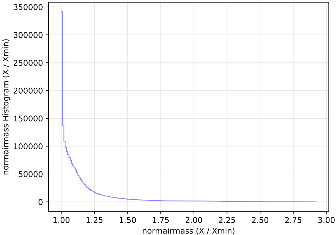
too_elab_r8_d2_griz_v3.4_10yrs All sky all bands: normairmass Histogram
