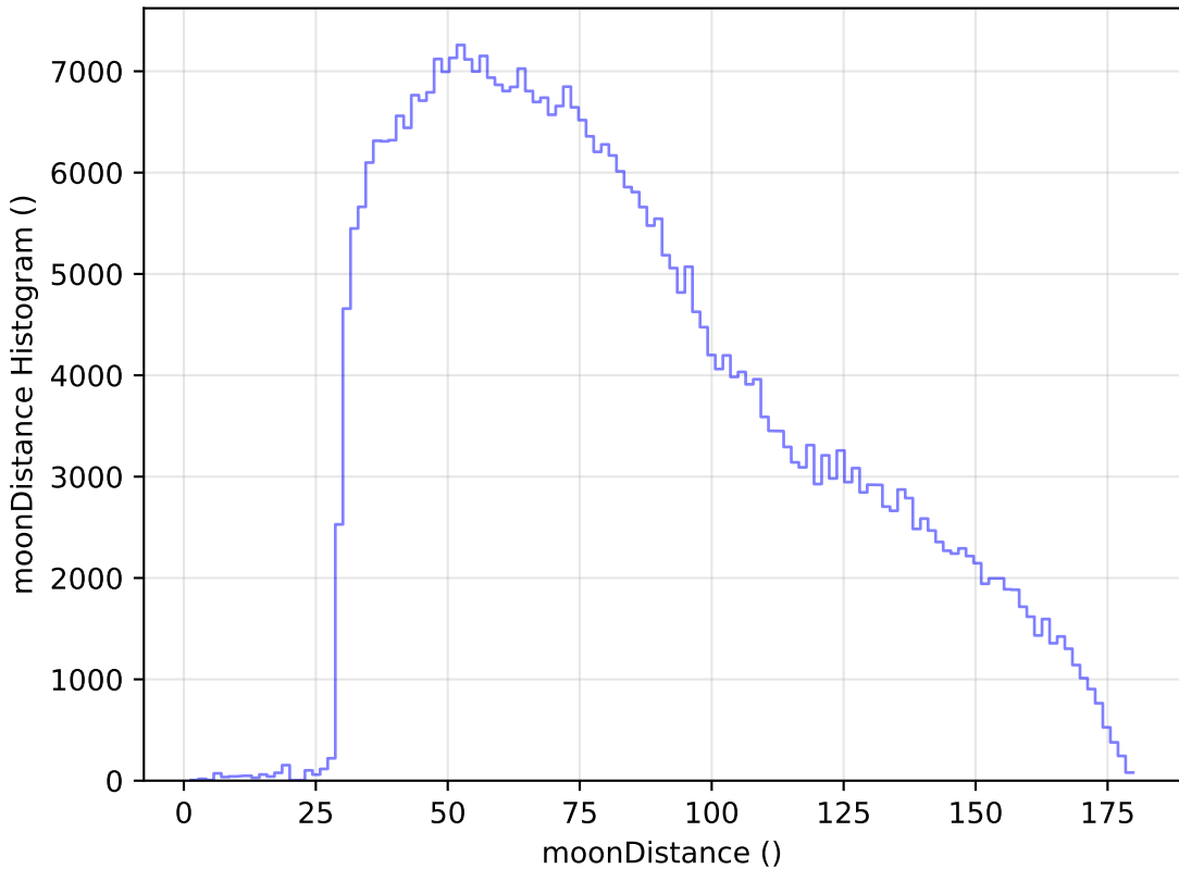
too_elab_r8_d2_griz_v3.4_10yrs WFD z band: moonDistance Histogram
