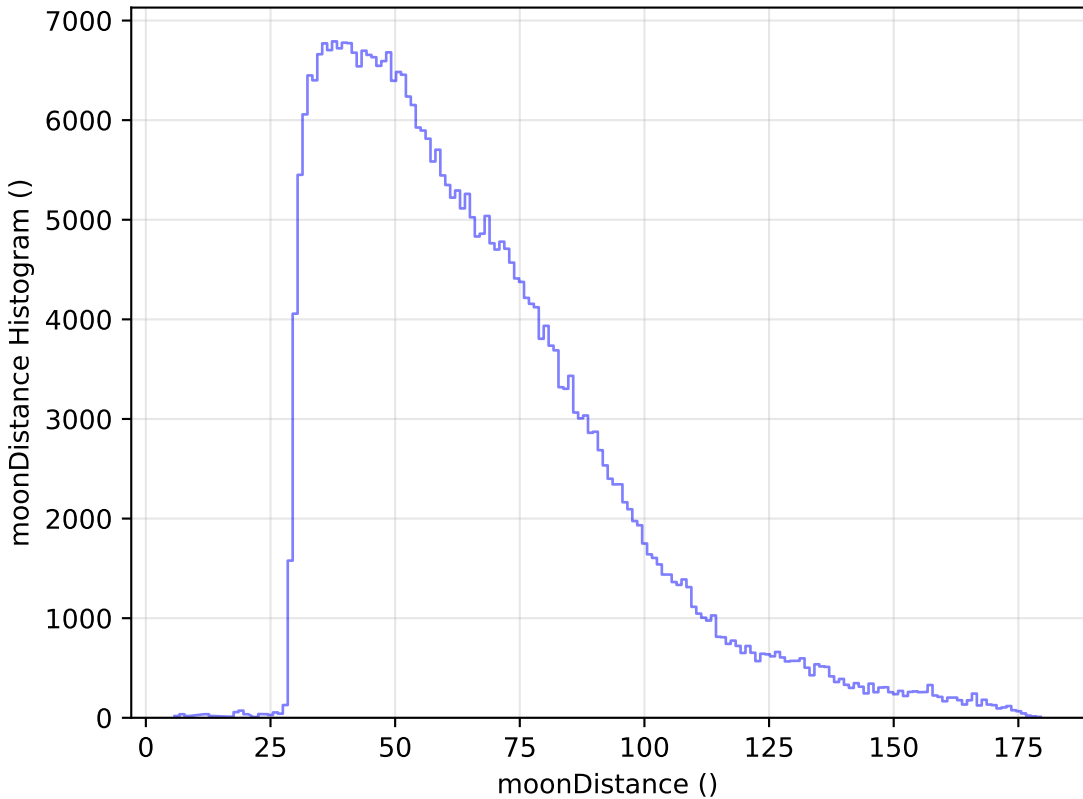
too_elab_r8_d2_griz_v3.4_10yrs WFD y band: moonDistance Histogram
