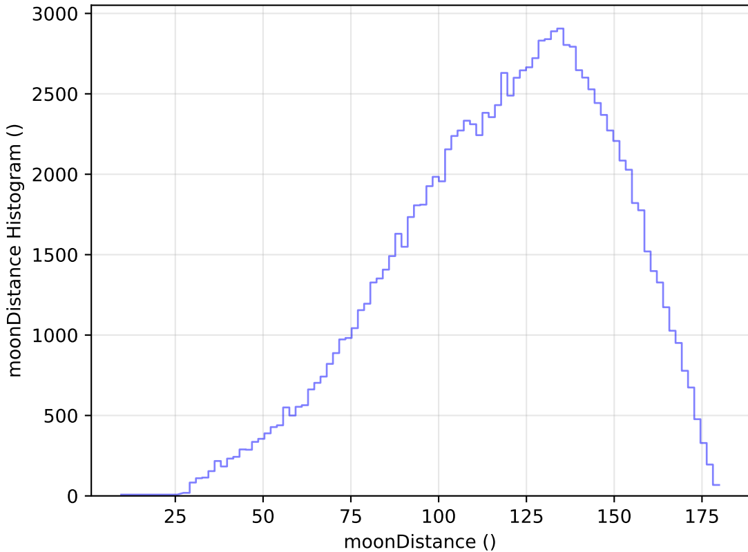
too_elab_r8_d2_griz_v3.4_10yrs WFD u band: moonDistance Histogram
