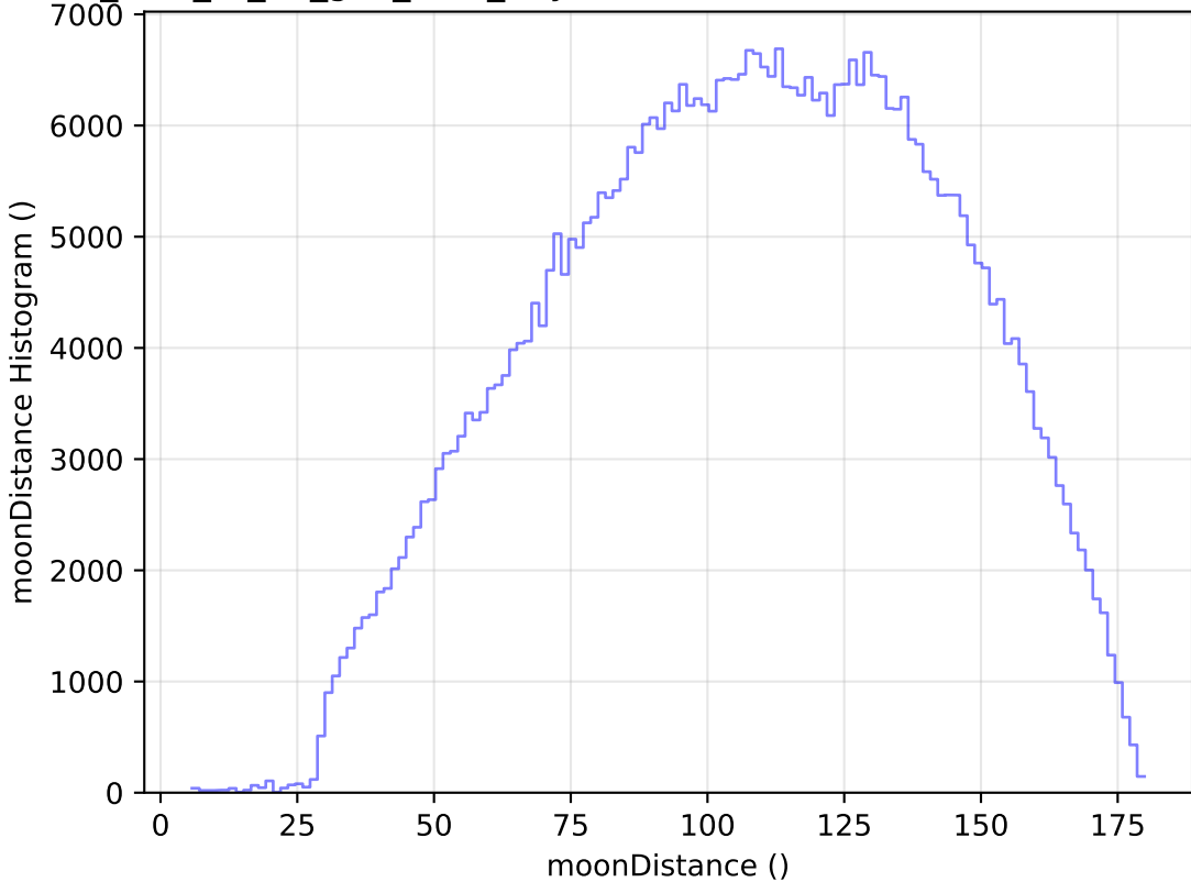
too_elab_r8_d2_griz_v3.4_10yrs WFD r band: moonDistance Histogram
