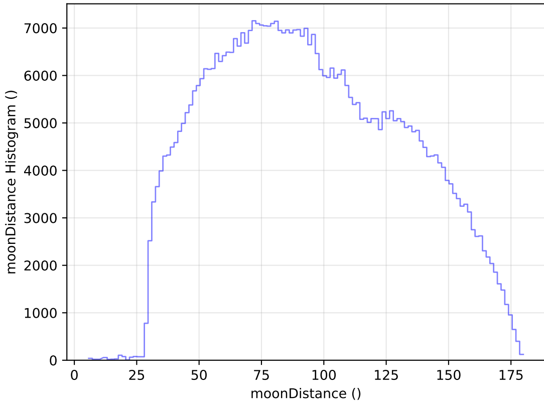
too_elab_r8_d2_griz_v3.4_10yrs WFD i band: moonDistance Histogram
