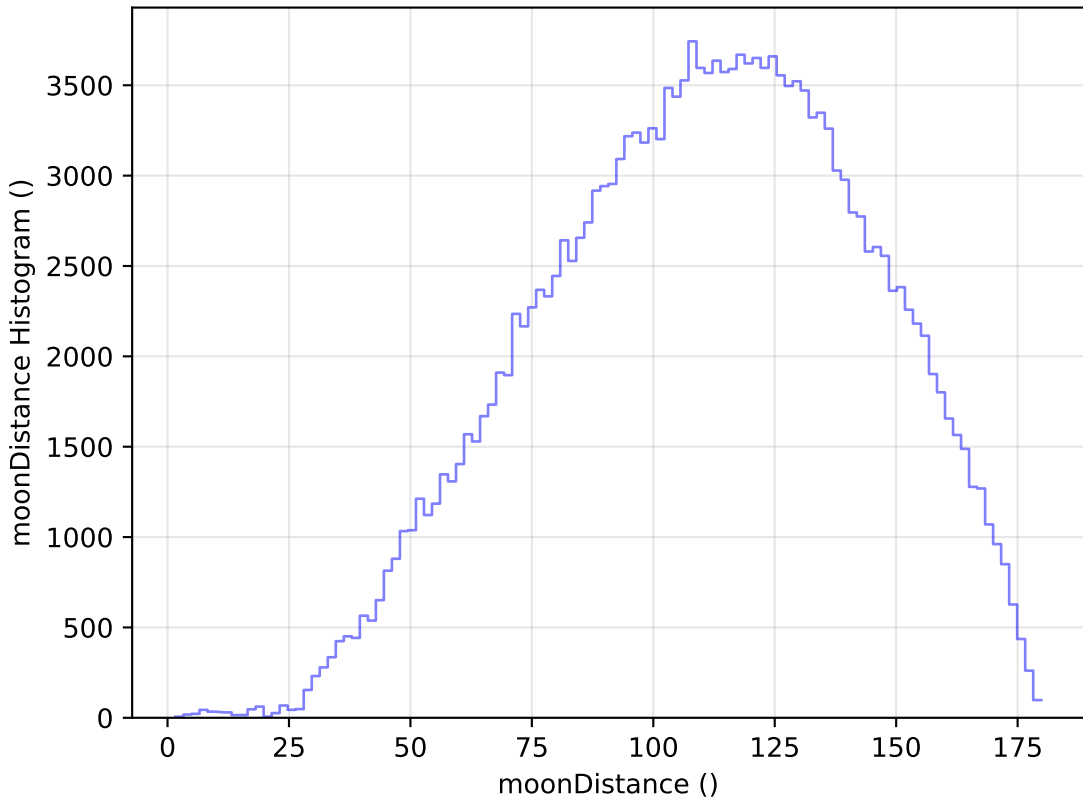
too_elab_r8_d2_griz_v3.4_10yrs WFD g band: moonDistance Histogram
