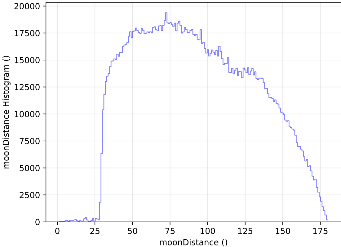
too_elab_r8_d2_griz_v3.4_10yrs WFD all bands: moonDistance Histogram
