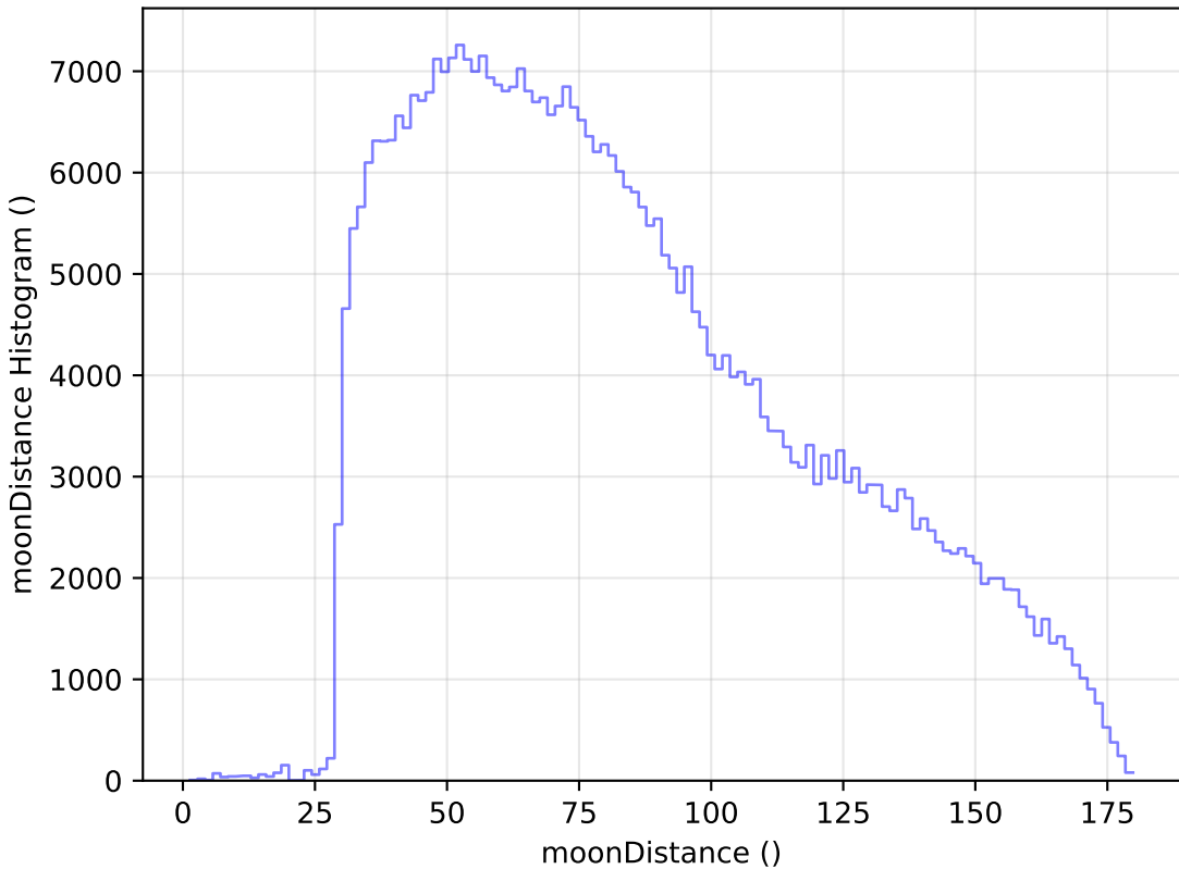
too_elab_r8_d2_griz_v3.4_10yrs All sky z band: moonDistance Histogram
