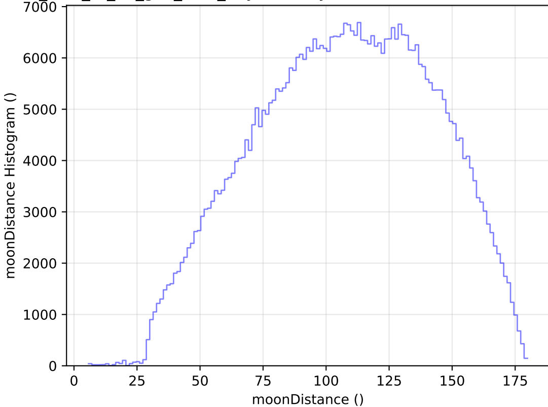
too_elab_r8_d2_griz_v3.4_10yrs All sky r band: moonDistance Histogram
