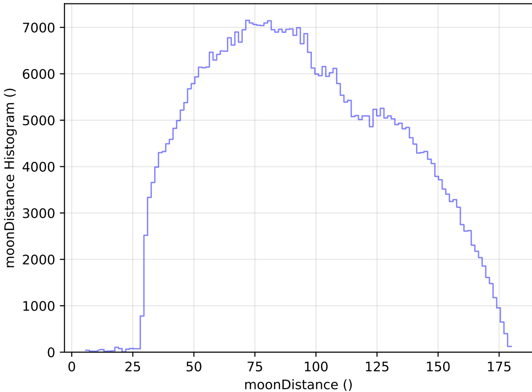
too_elab_r8_d2_griz_v3.4_10yrs All sky i band: moonDistance Histogram
