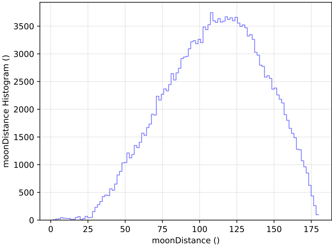
too_elab_r8_d2_griz_v3.4_10yrs All sky g band: moonDistance Histogram
