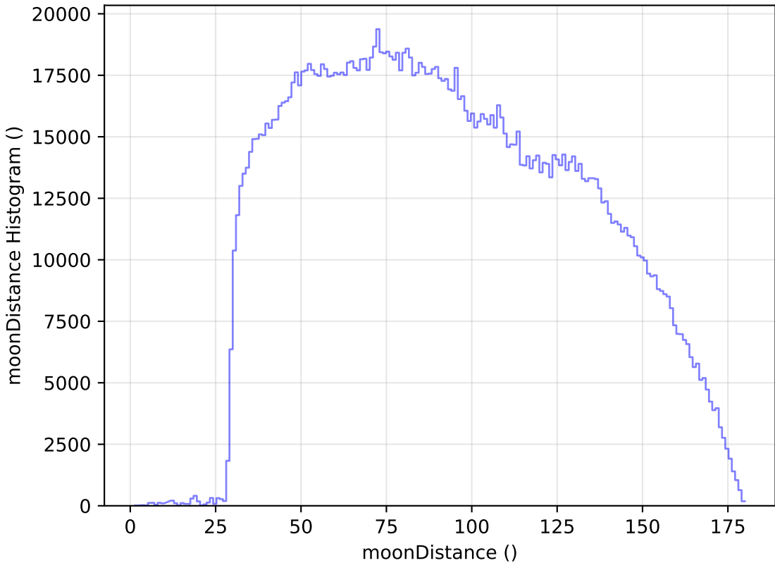
too_elab_r8_d2_griz_v3.4_10yrs All sky all bands: moonDistance Histogram
