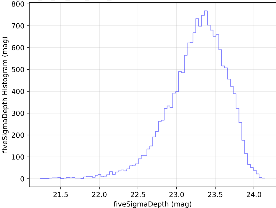
too_elab_r8_d2_griz_v3.4_10yrs Yr 1 u band: fiveSigmaDepth Histogram
