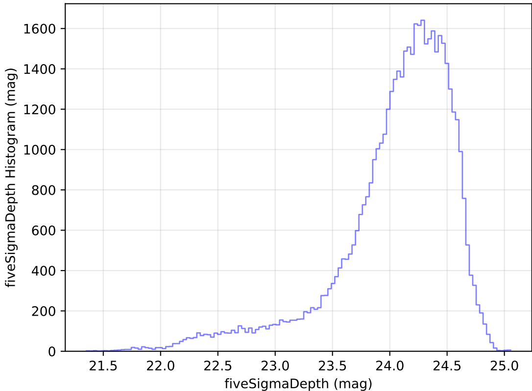
too_elab_r8_d2_griz_v3.4_10yrs Yr 1 r band: fiveSigmaDepth Histogram
