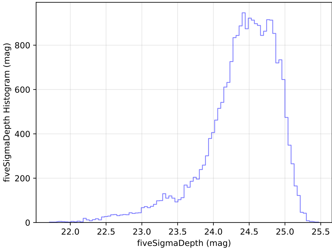
too_elab_r8_d2_griz_v3.4_10yrs Yr 1 g band: fiveSigmaDepth Histogram
