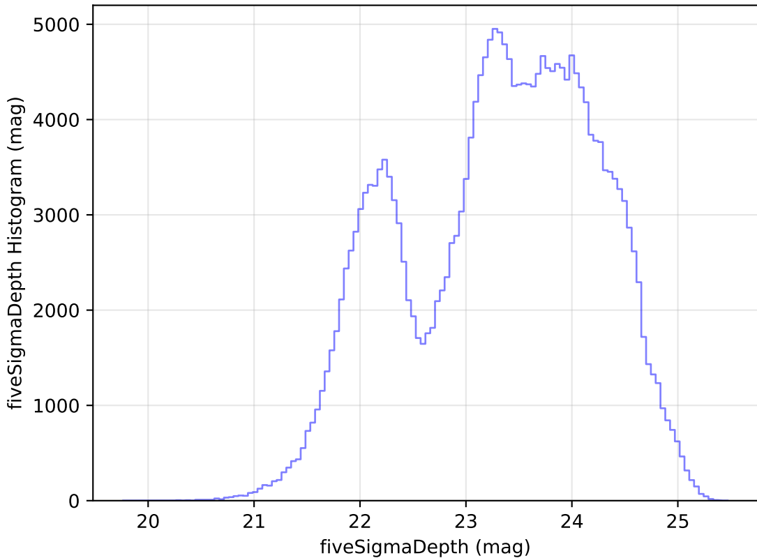
too_elab_r8_d2_griz_v3.4_10yrs Yr 1 all bands: fiveSigmaDepth Histogram
