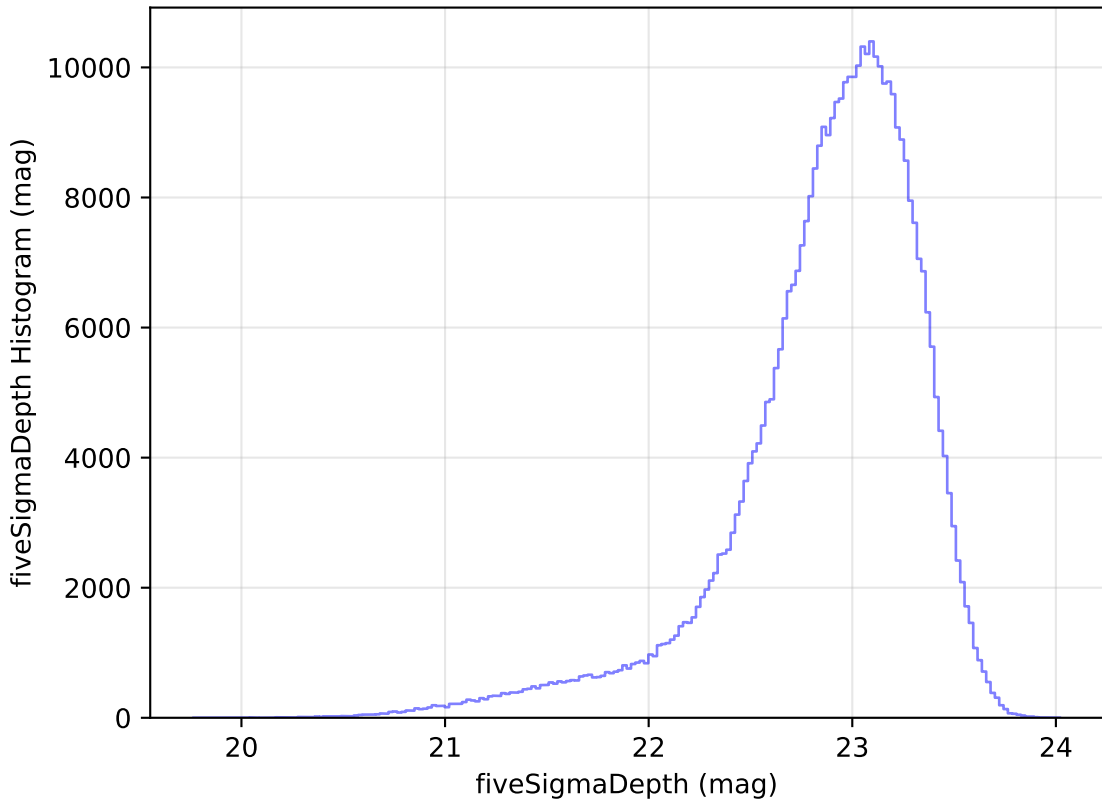
too_elab_r8_d2_griz_v3.4_10yrs WFD z band: fiveSigmaDepth Histogram
