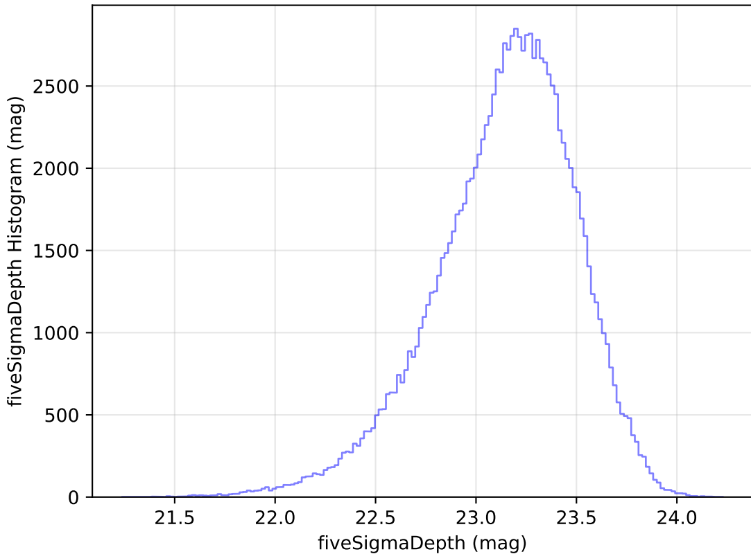
too_elab_r8_d2_griz_v3.4_10yrs WFD u band: fiveSigmaDepth Histogram
