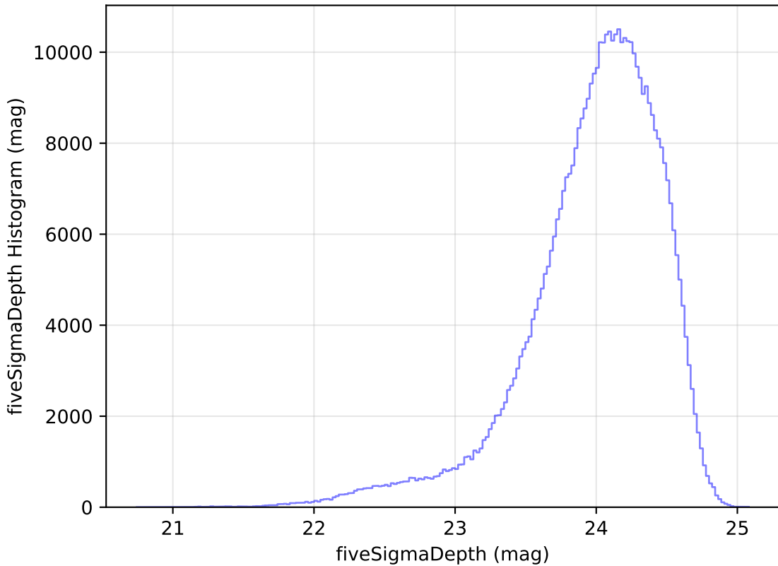
too_elab_r8_d2_griz_v3.4_10yrs WFD r band: fiveSigmaDepth Histogram
