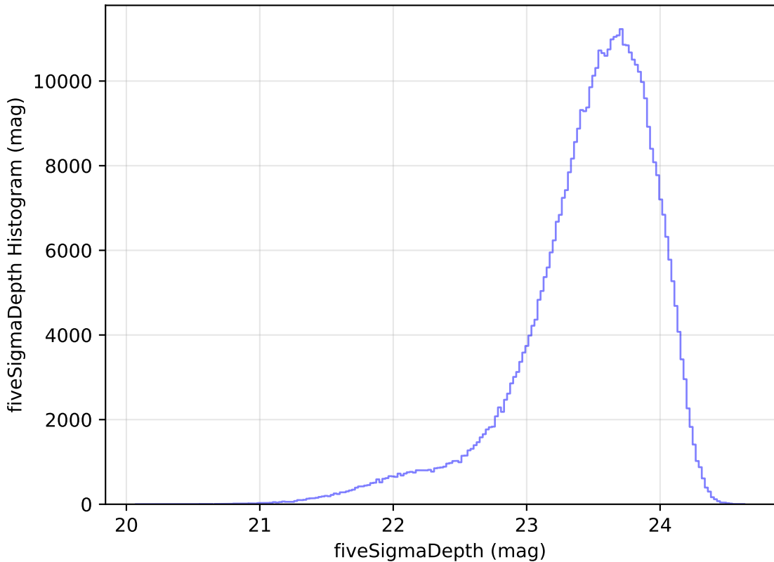
too_elab_r8_d2_griz_v3.4_10yrs WFD i band: fiveSigmaDepth Histogram
