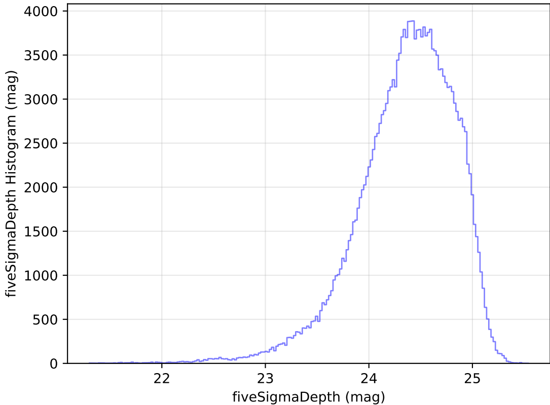
too_elab_r8_d2_griz_v3.4_10yrs WFD g band: fiveSigmaDepth Histogram
