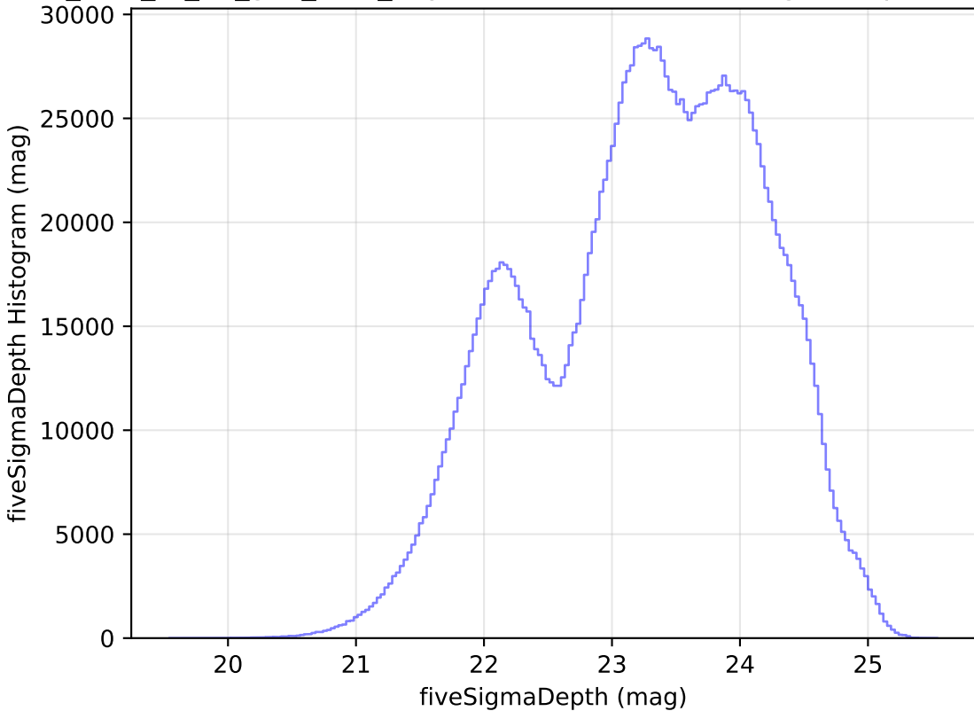
too_elab_r8_d2_griz_v3.4_10yrs WFD all bands: fiveSigmaDepth Histogram
