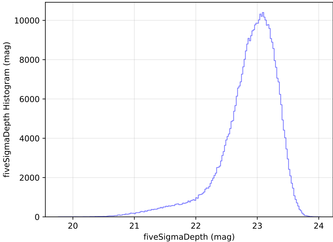
too_elab_r8_d2_griz_v3.4_10yrs All sky z band: fiveSigmaDepth Histogram
