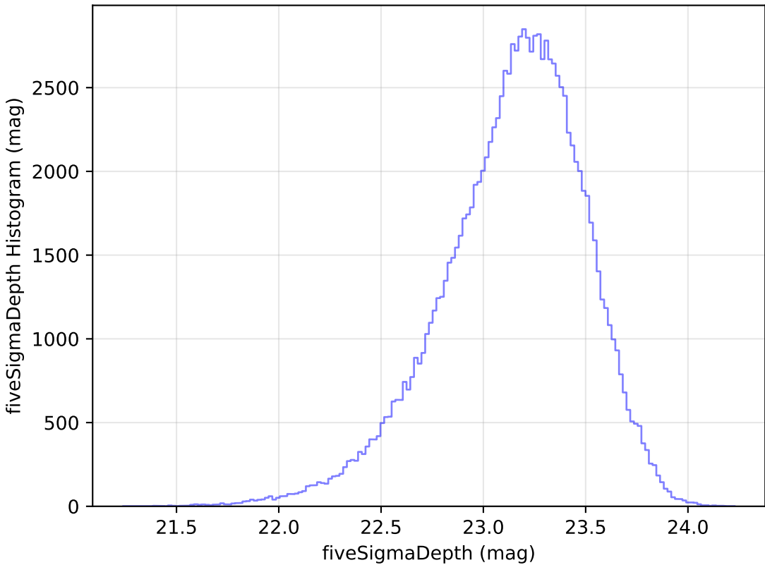
too_elab_r8_d2_griz_v3.4_10yrs All sky u band: fiveSigmaDepth Histogram
