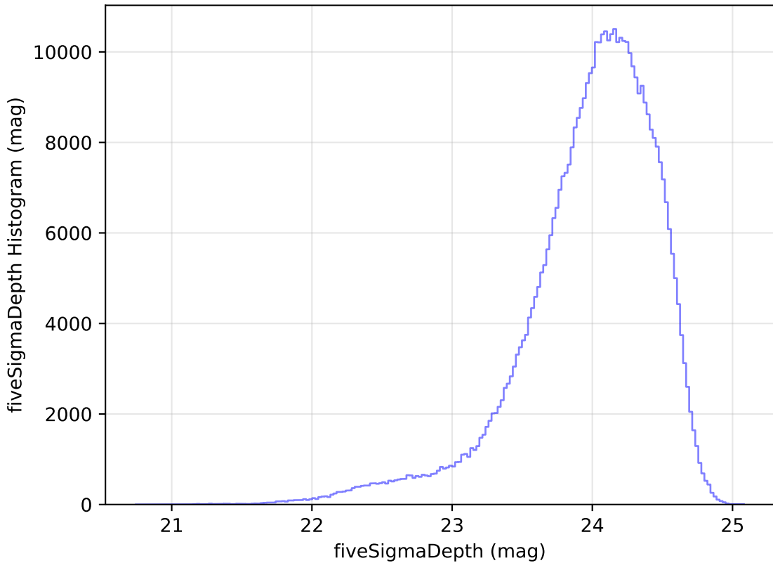
too_elab_r8_d2_griz_v3.4_10yrs All sky r band: fiveSigmaDepth Histogram
