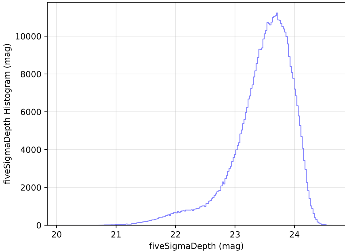
too_elab_r8_d2_griz_v3.4_10yrs All sky i band: fiveSigmaDepth Histogram
