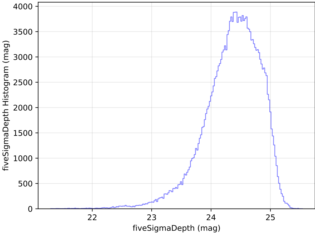
too_elab_r8_d2_griz_v3.4_10yrs All sky g band: fiveSigmaDepth Histogram
