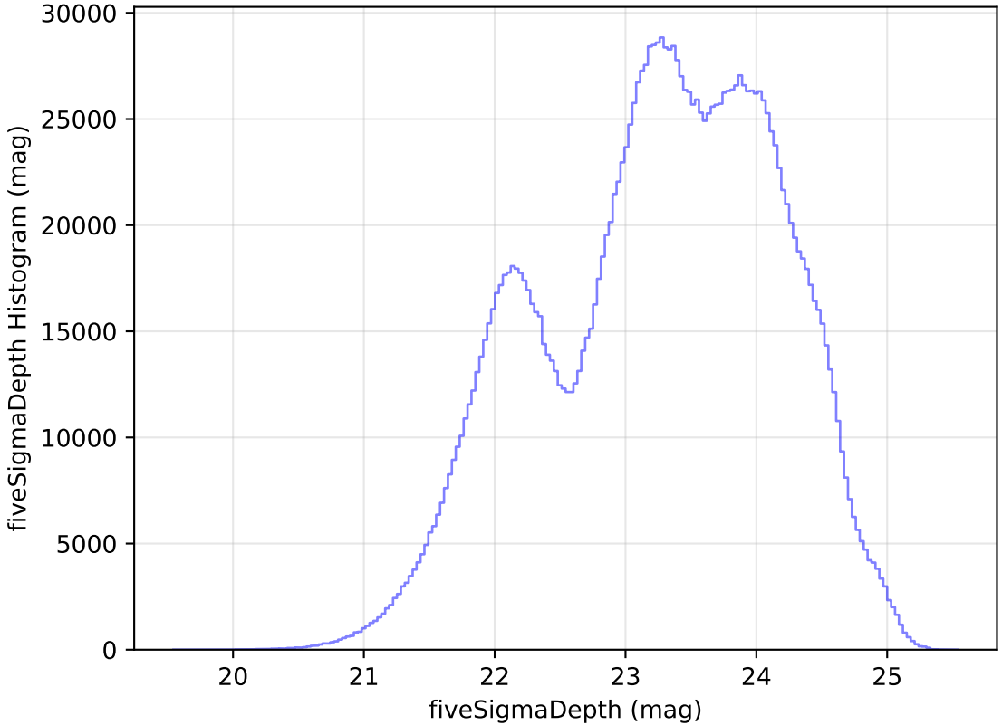
too_elab_r8_d2_griz_v3.4_10yrs All sky all bands: fiveSigmaDepth Histogram
