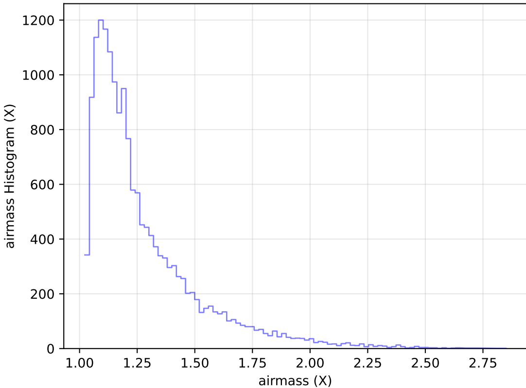
too_elab_r8_d2_griz_v3.4_10yrs Yr 1 u band: airmass Histogram
